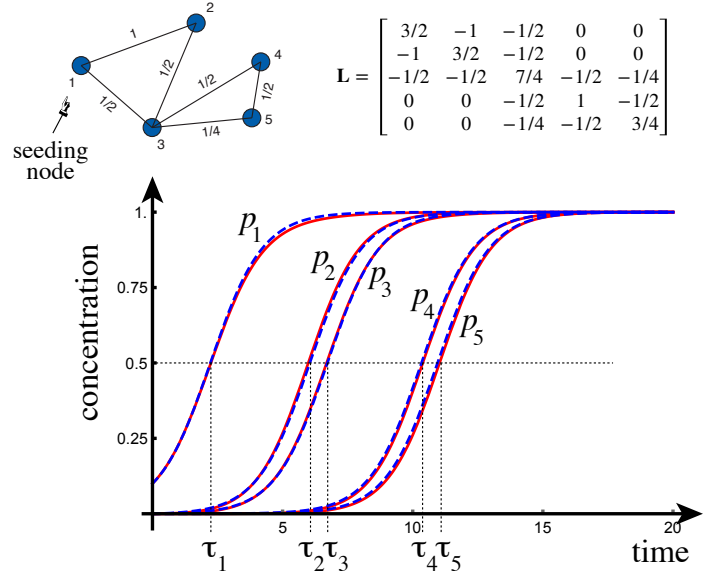
Figure 1: Example of dynamics on a 5-node network. Initially, only the first node is seeded ( p_1(0) = 1/10 ). Due to the coupling term, the second node and then all other nodes are invaded. The numerical solution is shown in red (solid) and the nonlinear asymptotic solution are in blue (dashed) ( \alpha = 1 , \rho = 1/100 ).
